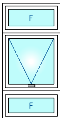
JANELA MAXIM-AR VERTICAL C/ 2 BAND FX
